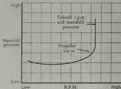
FIGURE 10-43. Effect of propeller governor on manifold pressure.
